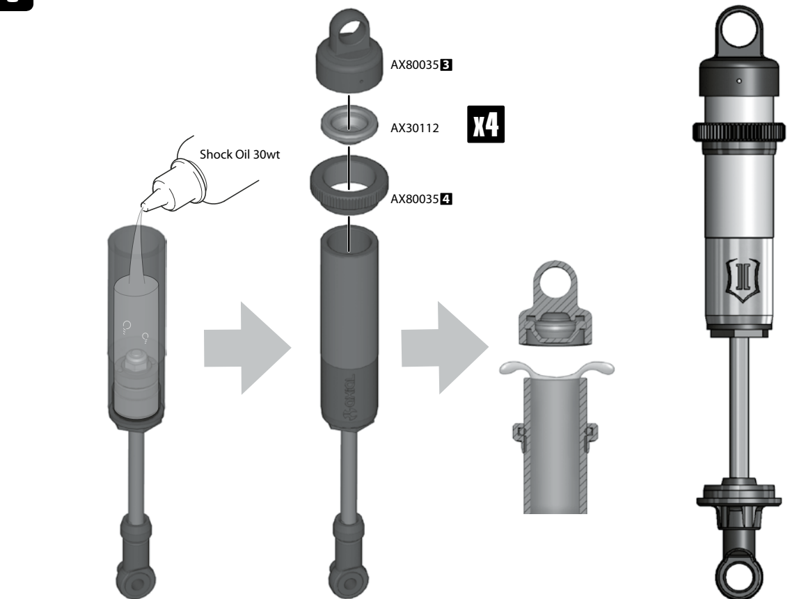
AX31188 Aluminum Shock Body 12x47.5mm x4
